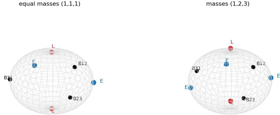
Fig. 1 The shape sphere: 3 Euler (E), 2 Lagrange (L), 3 binary-collision rays (B). Masses move the points; they never change the count.
